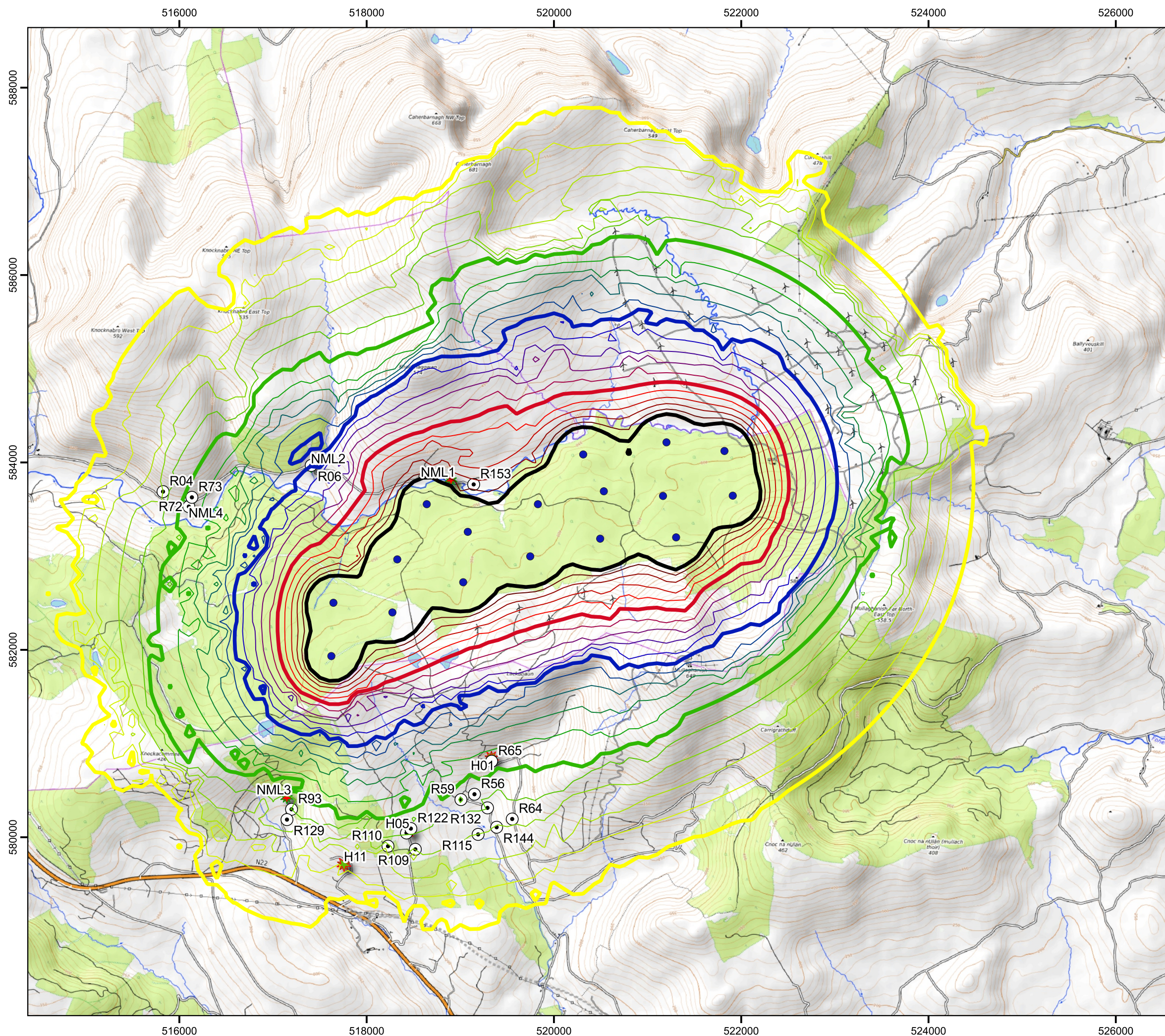
Figure 13-1 Predicted Operational Noise Levels at Rated Power - Proposed Development Only
